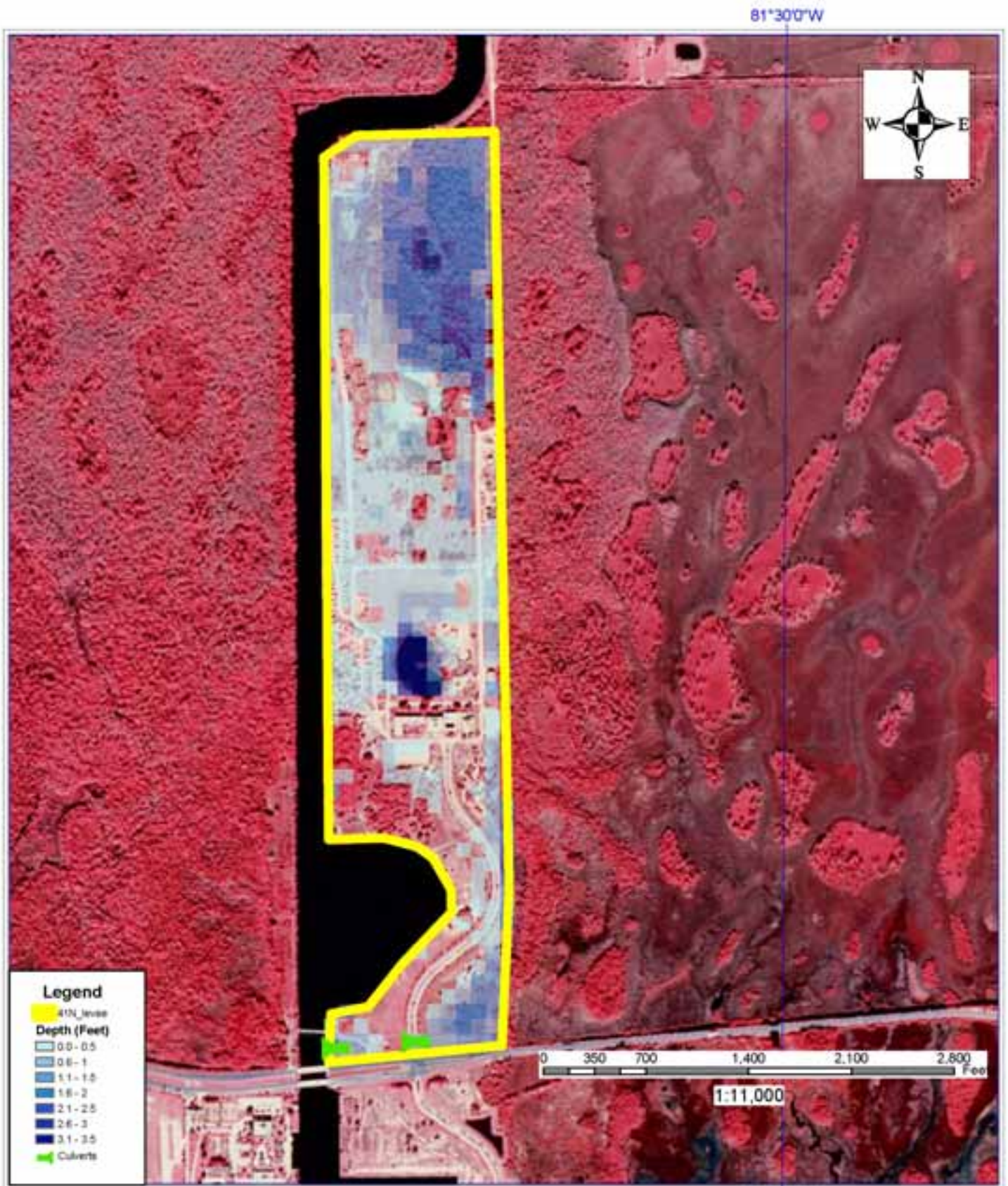
Figure A-192. 41 North Levee {41 N Levee} Residual Flooded Areas for 25-year Design Storm
