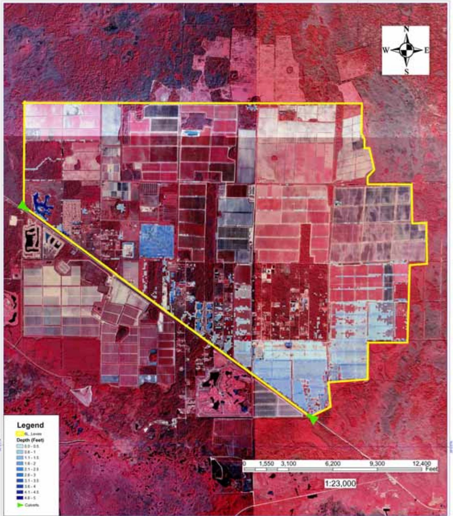
Figure A-191. 6L Levee (6L Levee) Residual Flooded Areas for 25-year Design Storm
