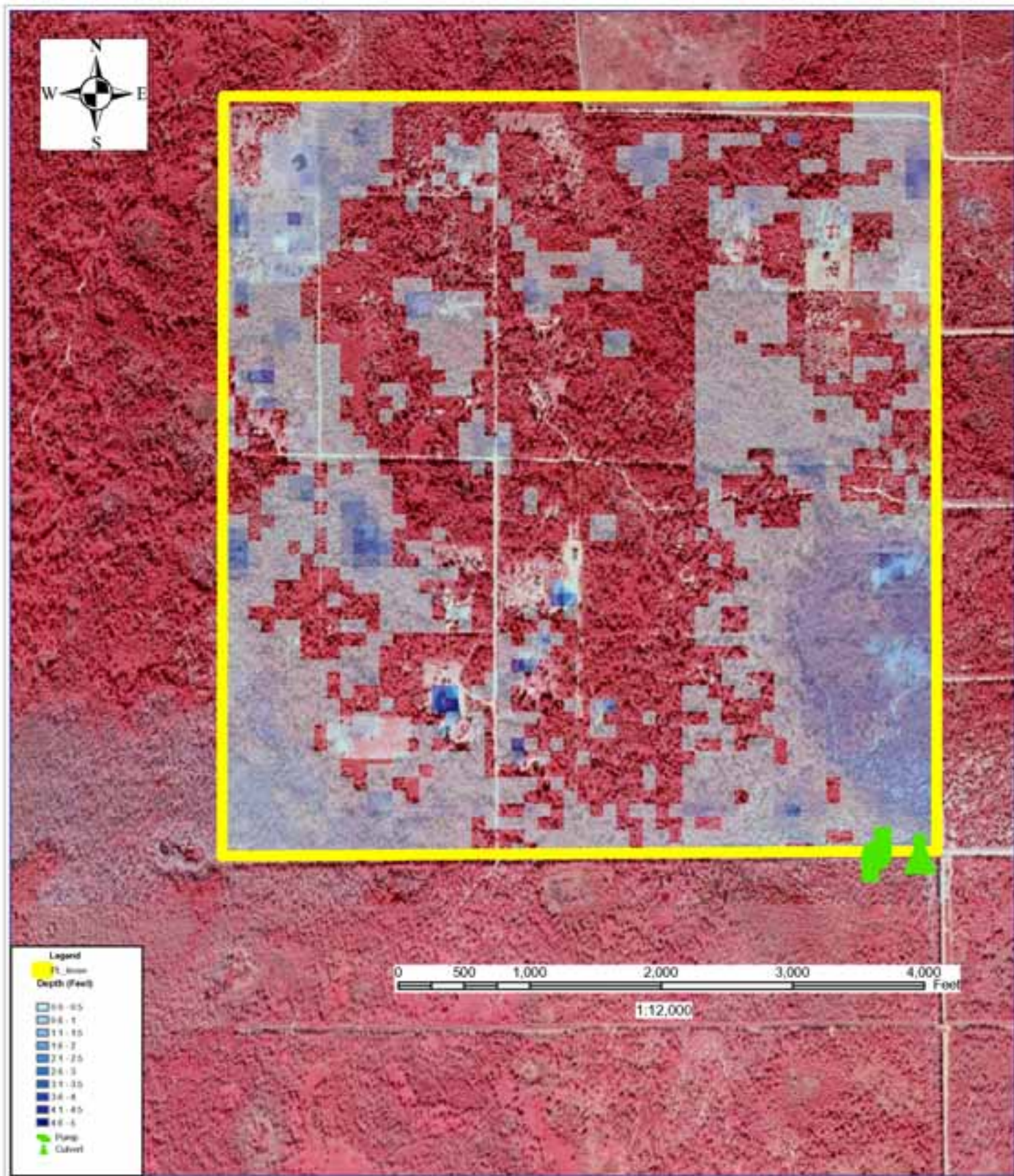
Figure A195. Private Lands Levee (PL Levee) Residual Flooded Areas for 25-year Design Storm
