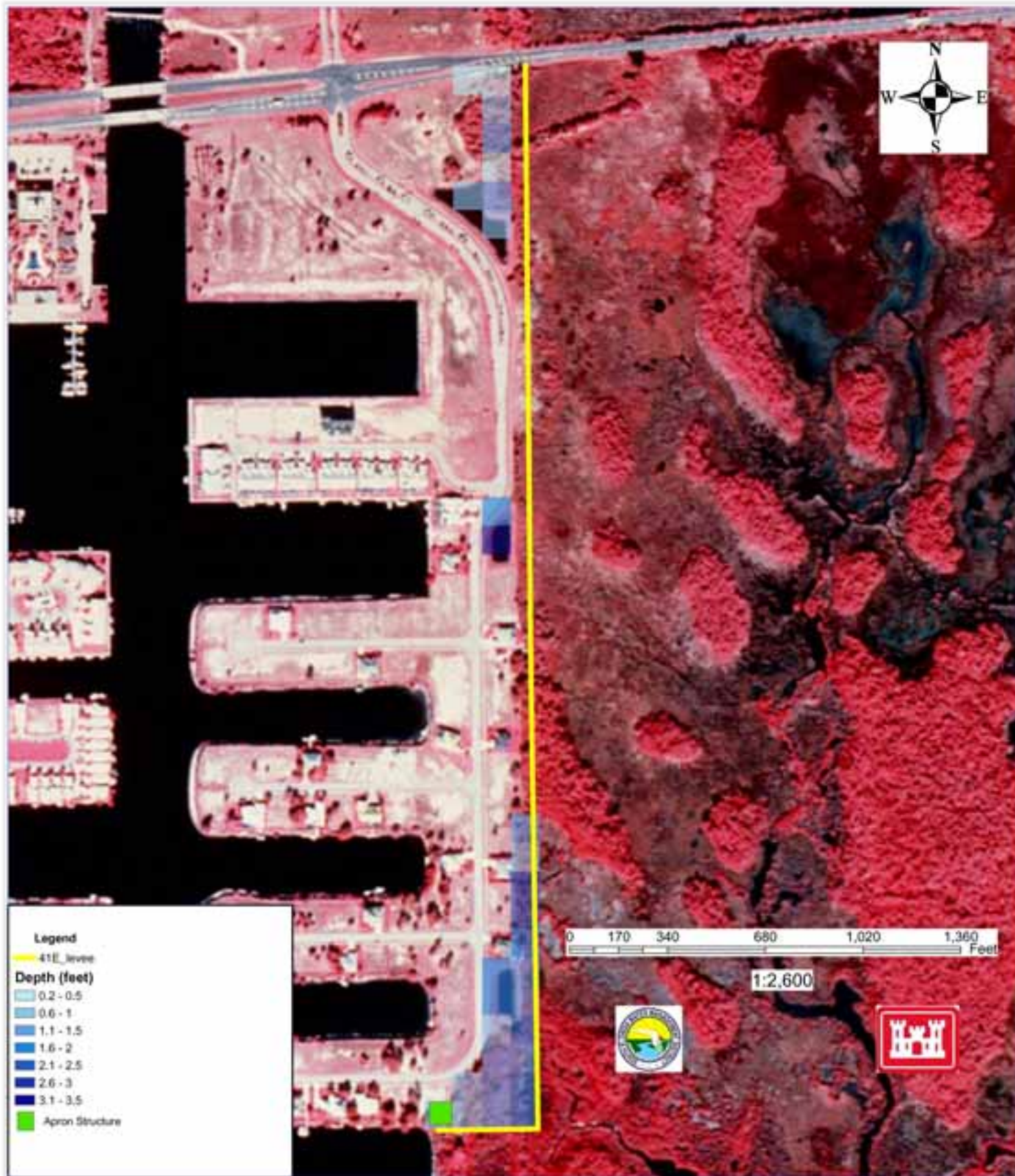
Figure A-193. 41 East Levee Residual Flooded Areas for 25-year Design Storm
