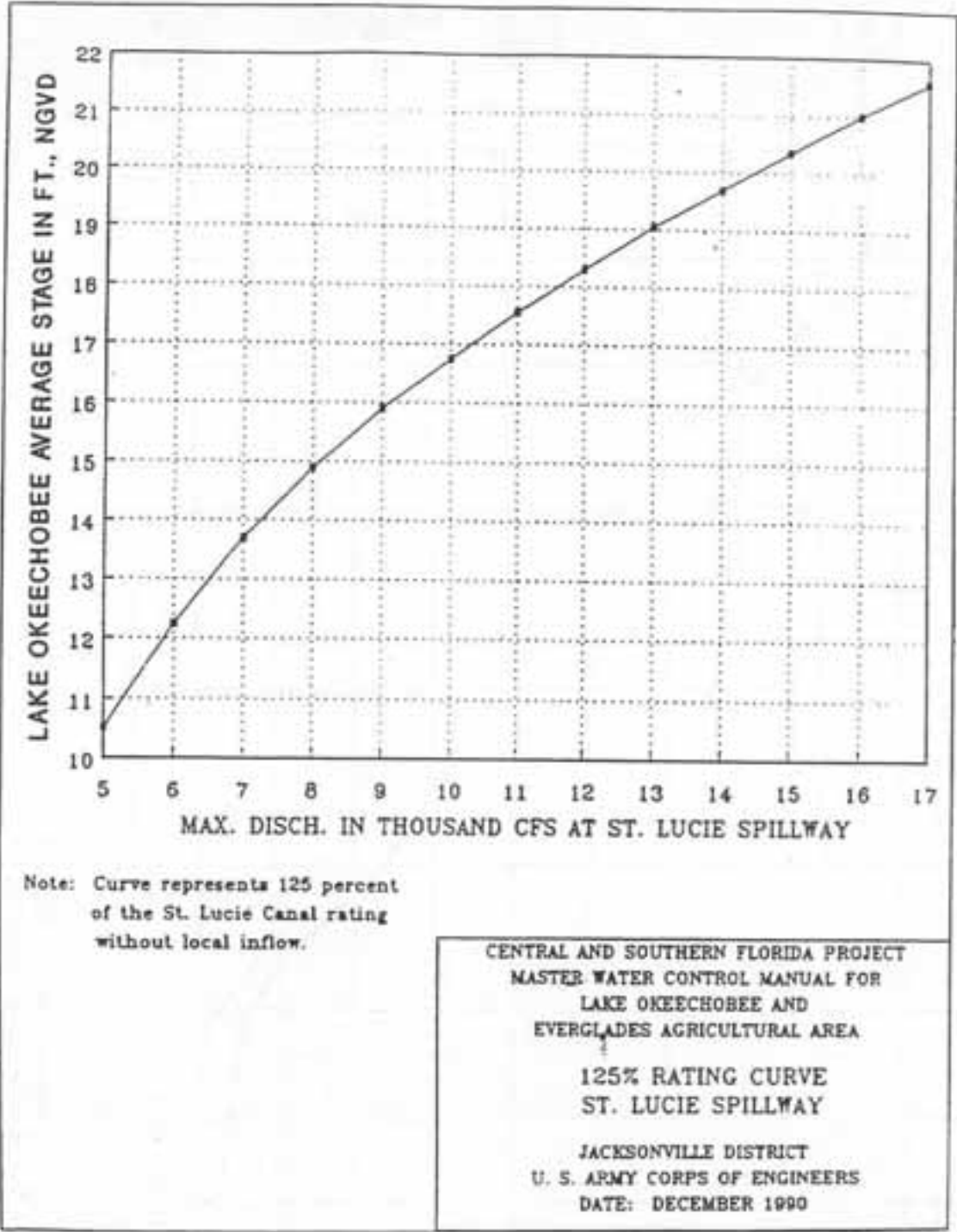
FIGURE 7-3 ST. LUCIE SPILLWAY 125% RATING CURVE
