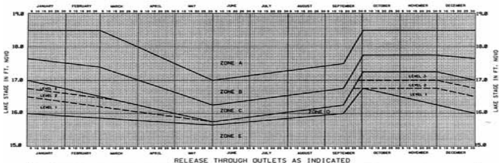
FIGURE 3-8 INTERIM REGULATION SCHEDULE 1994 – RUN 25
