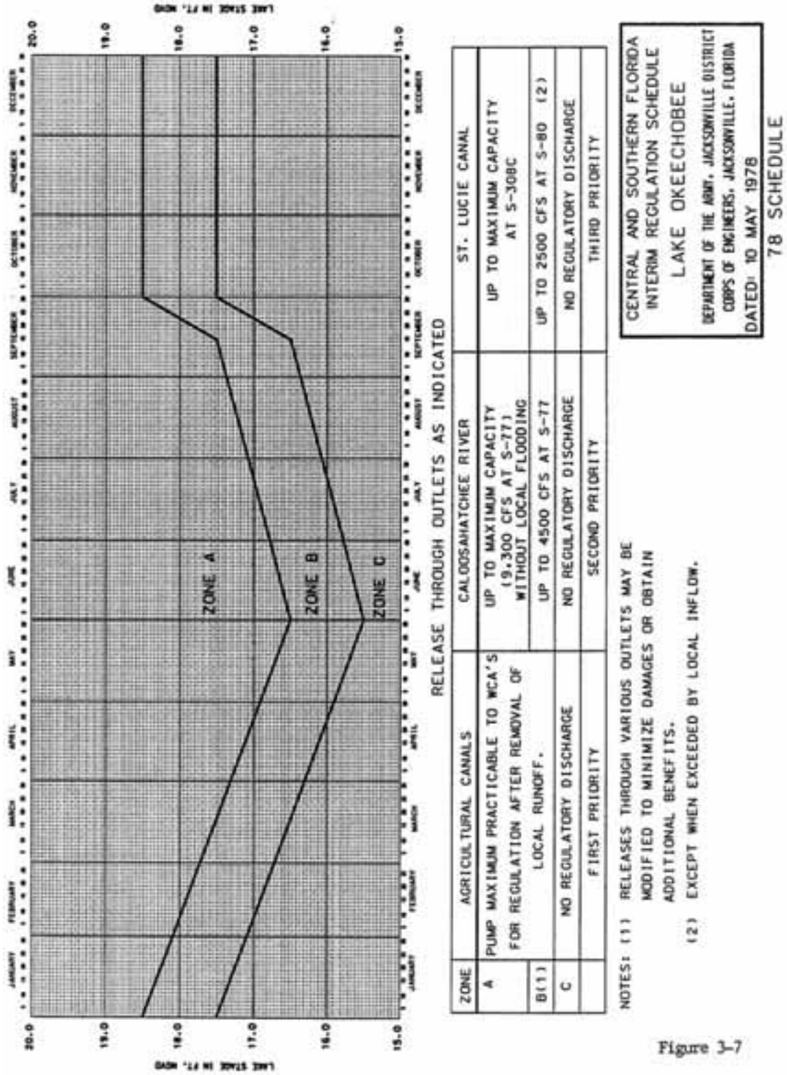
FIGURE 3-7 INTERIM REGULATION SCHEDULE 1978
